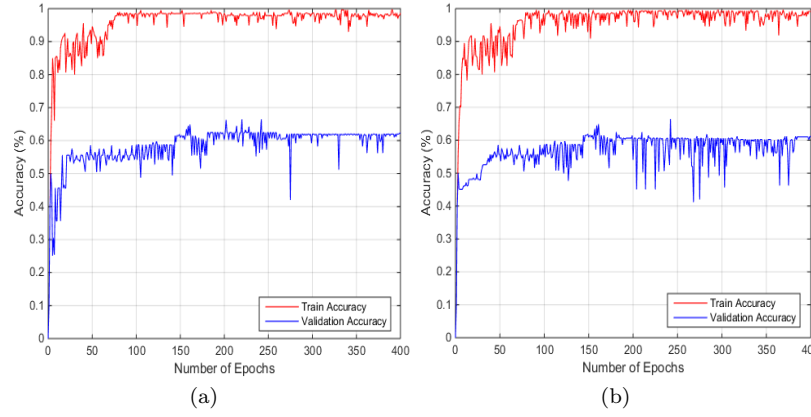
Fig. 9 Performance [Accuracy] with number of epochs with different states using CNN Model.: (a) EO Vs Task2 (b) and EC Vs Task2.
