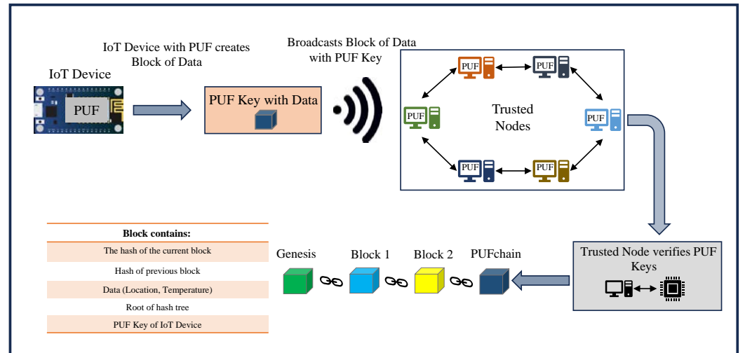
(a) PUFchain
