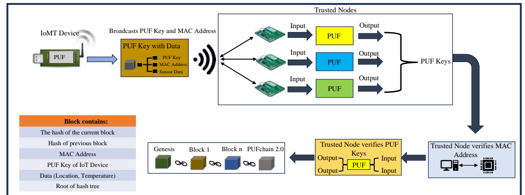
(b) PUFchain 2.0
