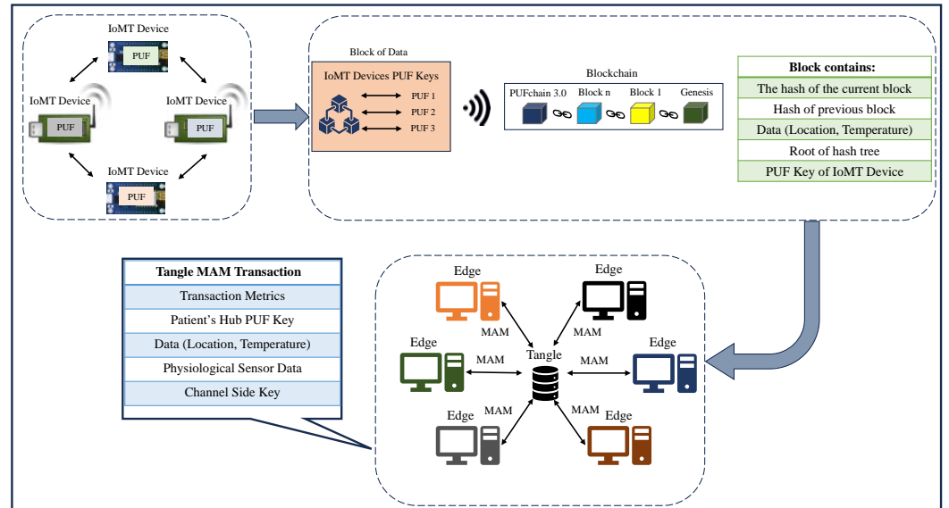
(c) Proposed PUFchain 3.0
