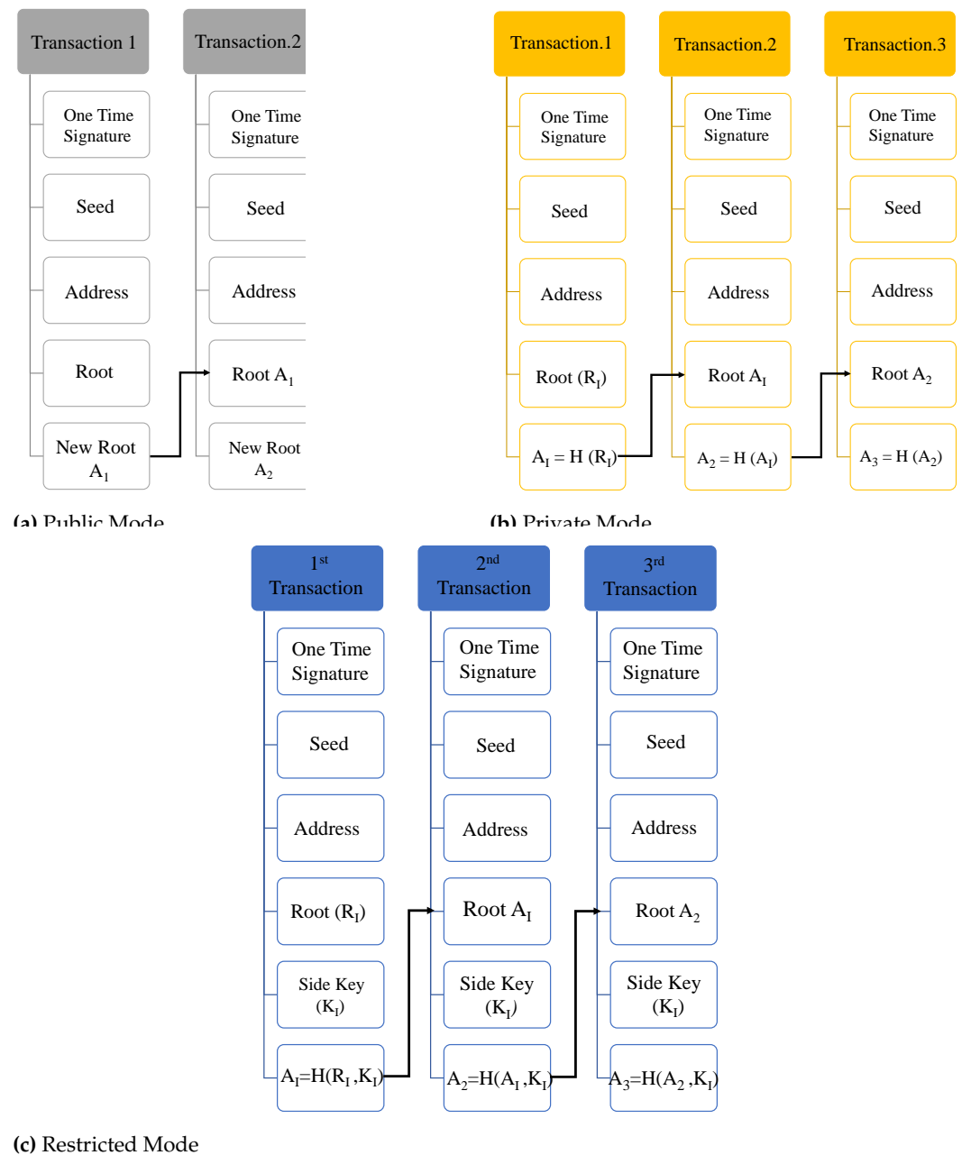
Figure 8. Masked Authentication Messaging
