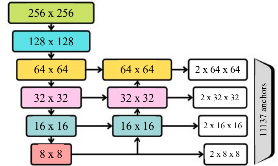
Fig. 3. Comprehensive View: Gesture Recognition Module Architecture
