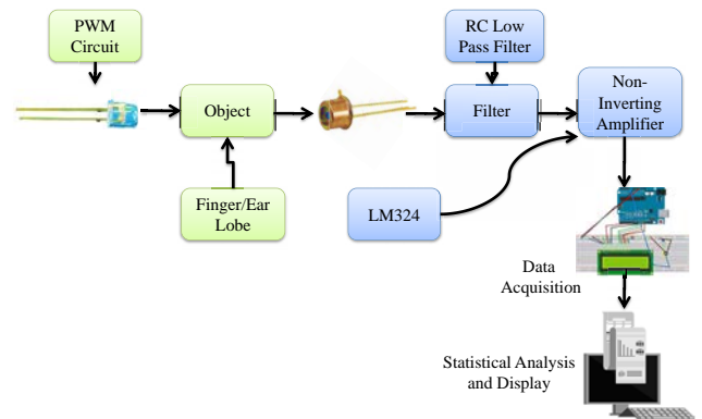
FIGURE 16: Block diagram representation of IR spectroscopy.
