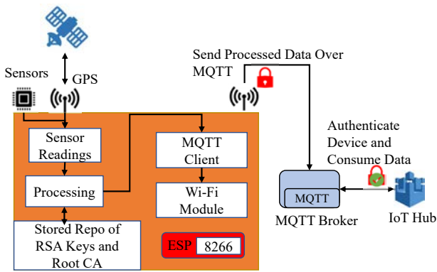
Fig. 5: Proposed Sensing Node Sharing Data Securely to Cloud
