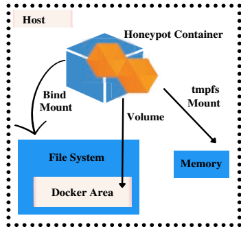
Figure 7: Storage Pathways of Bind Mount, Volume, and tmpfs Mount in Docker Linux Honeypots
