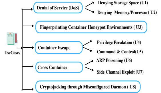
Figure 6: Usecase Observations Assembled by Research Findings
