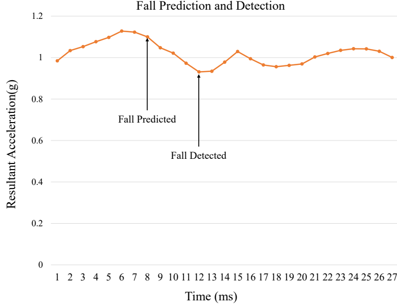
Figure 7. Fall detection and Prediction.
