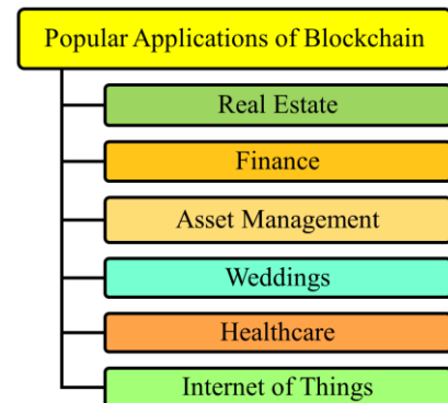
FIGURE 8. Blockchain applications.
