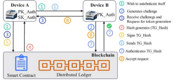
Fig. 3: Device authentication using SSI
