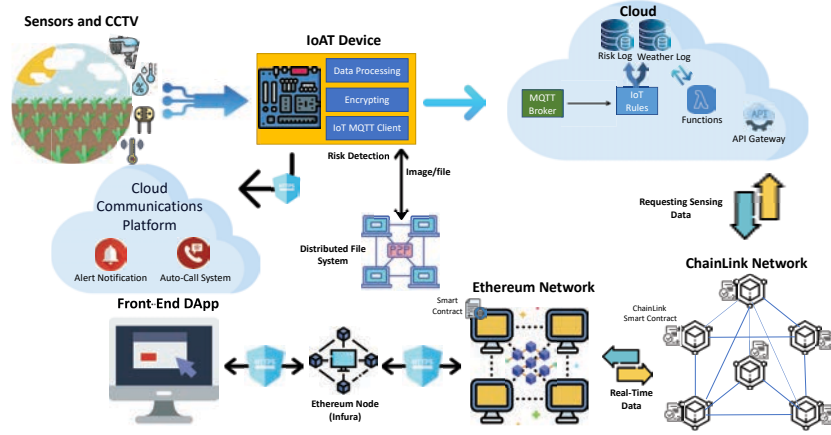
Fig. 1: FarmIns Architecture.
