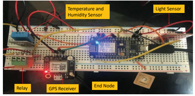
Fig. 3. Implemented End Node for Proposed PharmaChain 2.0.
