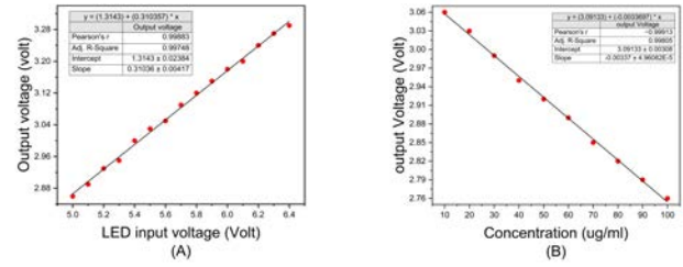
Fig. 3: Amplifier output voltage measurement at (A) different LED input voltage (B) different concentrations of nitrate solutions.
