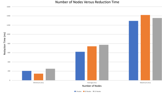
(b) Block Reduction Time.
