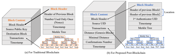
Fig. 4: The structure of block in the proposed post-blockchain.
