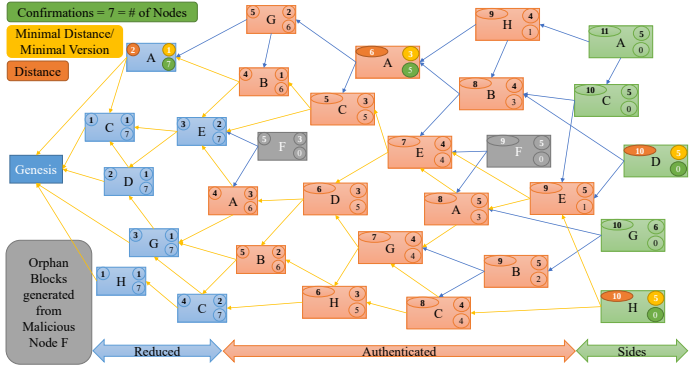
Fig. 5: Illustration of actions of the proposed McPoRA Algorithm in post-blockchain.
