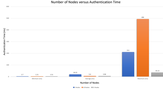
(a) Block Authentication Time.
